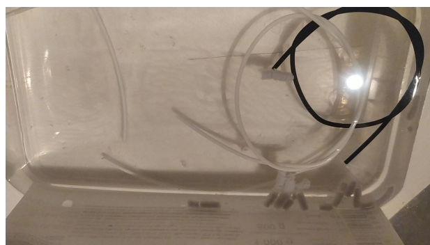
Figure 7: Testing ASA (white), ABS (ivory), PLA (grey) and TPU (black). The PLA was desolved the next day
