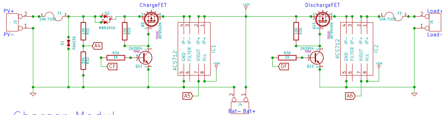
Charger Modul
