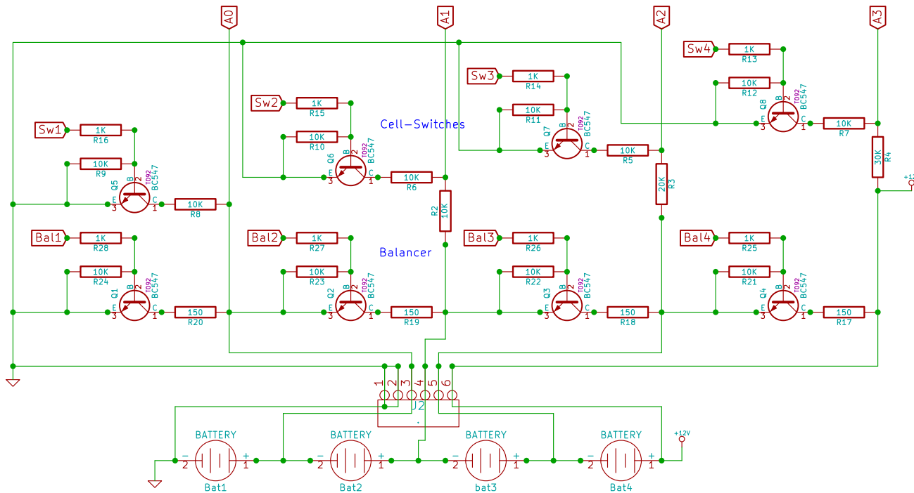
Balancer Modul
