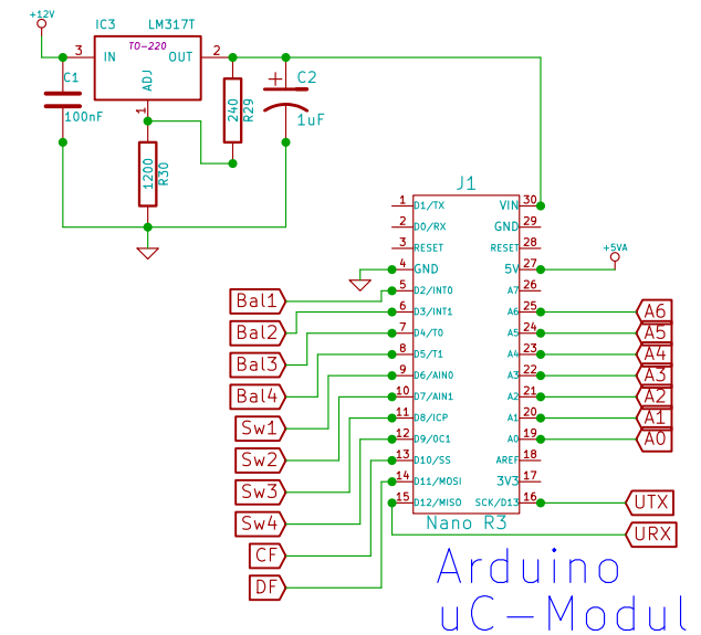
Data-Sampling Modul
